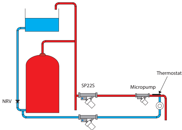
Diagram 32.2 If you want to boost the flow and pressure as well as recirculation add a SP22S to the flow and return as shown
