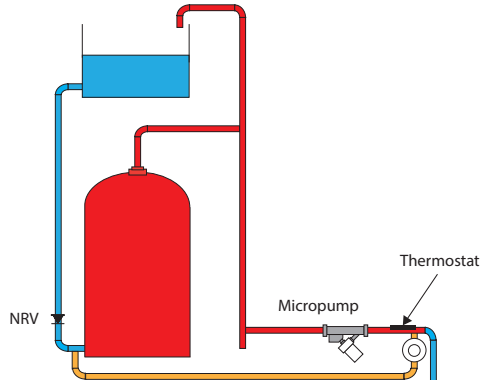
Diagram 32.1 This diagram above illustrates the components and the temperature of the pipes when hot water recirculation is active
